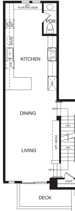
SECOND FLOOR
